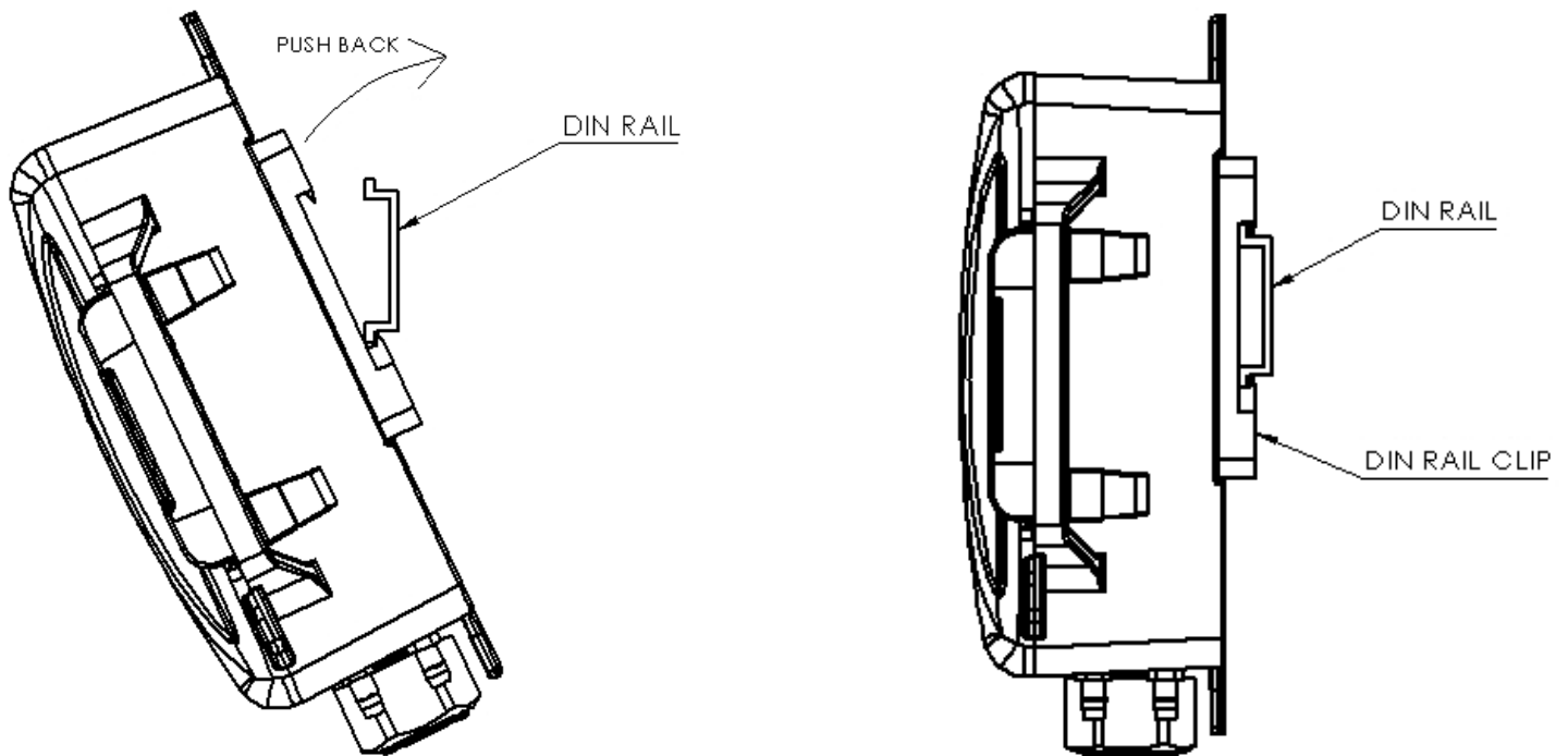
Figure 2: DIN Rail Mounting
